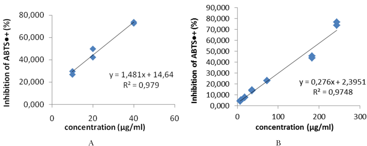
Fig. 3. The ability of A – quercetin, B – trolox scavenges ABTS radical cation. \text{IC}_{50} value of quercetin is (24 \pm 1) \mu\text{g}/\text{ml} . \text{IC}_{50} value of trolox is (170.1 \pm 0.1) \mu\text{g}/\text{ml} . Results are means \pm SD ( n = 2 ).
