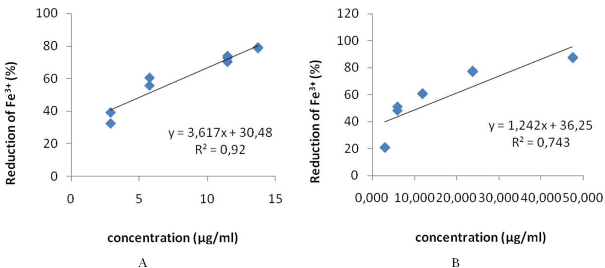
Fig. 5. The ability of A – quercetin, B – trolox to reduce Fe 3+ . IC 50 value of quercetin is 5.40 µg/ml ± 0.03. IC 50 value of trolox is 11.1 µg/ml ± 0.7. Results are means ± SD (n = 2).
