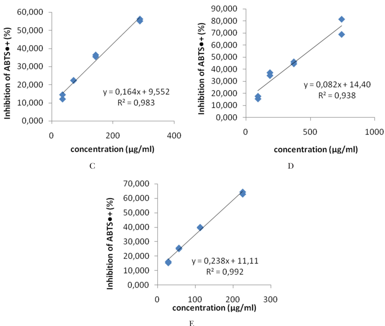
Fig. 4. The ability of C – curcumin-cyclodextrin complex, D – curcumin-phospholipid complex, E – curcuminoids scavenges ABTS radical cation. IC 50 value of curcumin-cyclodextrin complex is (246 ± 1) µg/ml. IC 50 value of curcumin-phospholipid complex is (430 ± 1) µg/ml. IC 50 value of curcuminoids is (163.4 ± 0.6) µg/ml. Results are means ± SD (n = 2).
