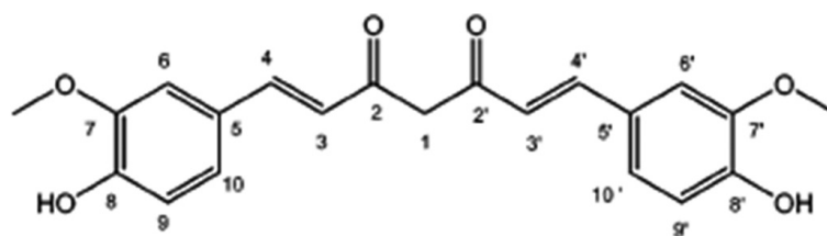
Fig. 1. Chemical structure of curcumin (Payton et al., 2007).
