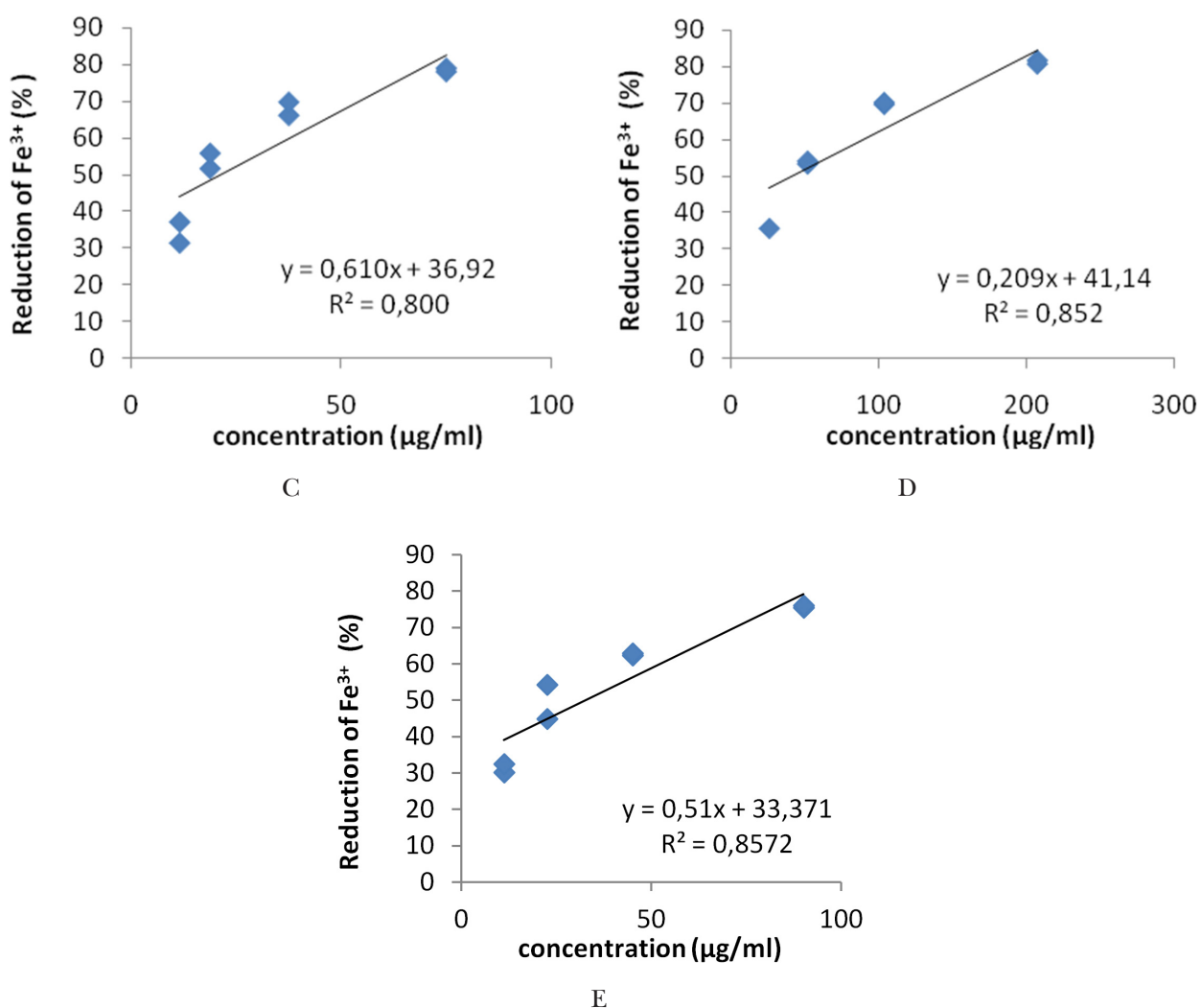
Fig. 6. The ability of C – curcumin-cyclodextrin complex, D – curcumin-phospholipid complex, E – curcuminoids to reduce Fe 3+ . IC 50 value of curcumin-cyclodextrin complex is 21.4 µg/ml ± 0.7. IC 50 value of curcumin-phospholipid complex is 42.3 µg/ml ± 0.5. IC 50 value of curcuminoids is 32.6 µg/ml ± 2.3. Results are means ± SD (n = 2).
